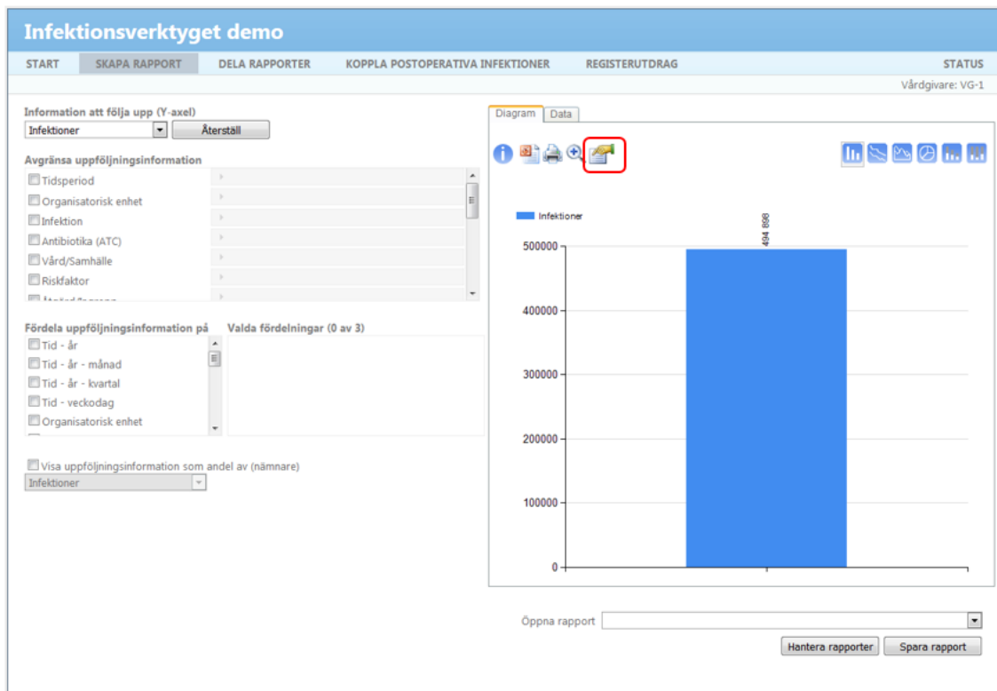
Figur 8 Formatera diagram
