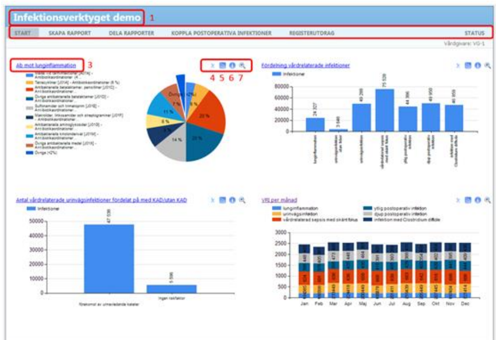
Figur 3 Startside.
