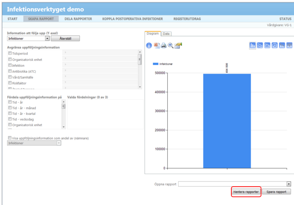
Figur 11 Hantera rapporter.
